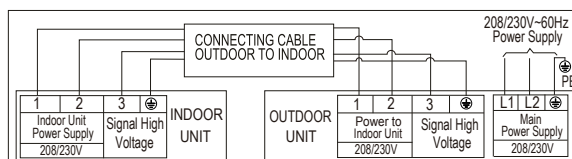
Connection Diagram
