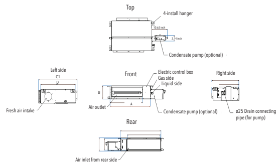
External Pump
